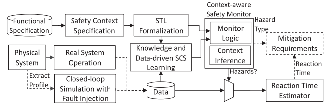
Fig. 2. Framework for design of context-aware monitors.
